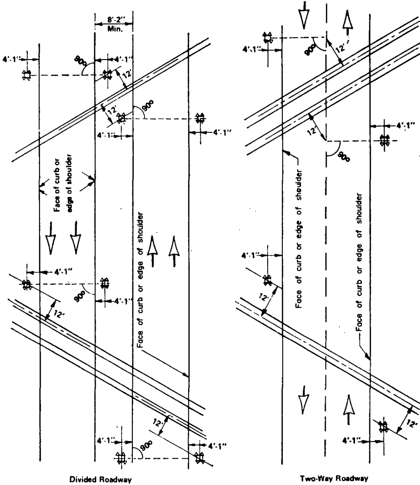
STANDARD RAILROAD CROSSING SIGNAL LOCATIONS
