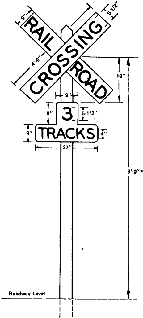
RAILROAD CROSSBUCK SIGN
