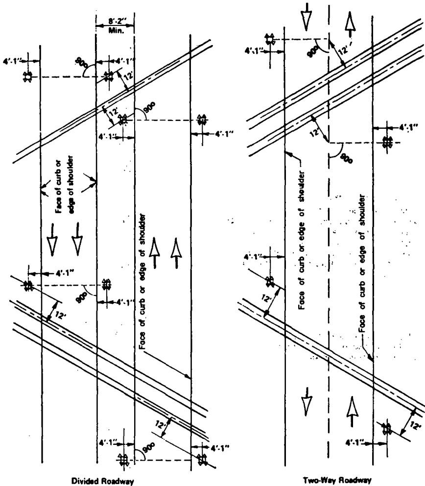
STANDARD RAILROAD CROSSING SIGNAL LOCATIONS
