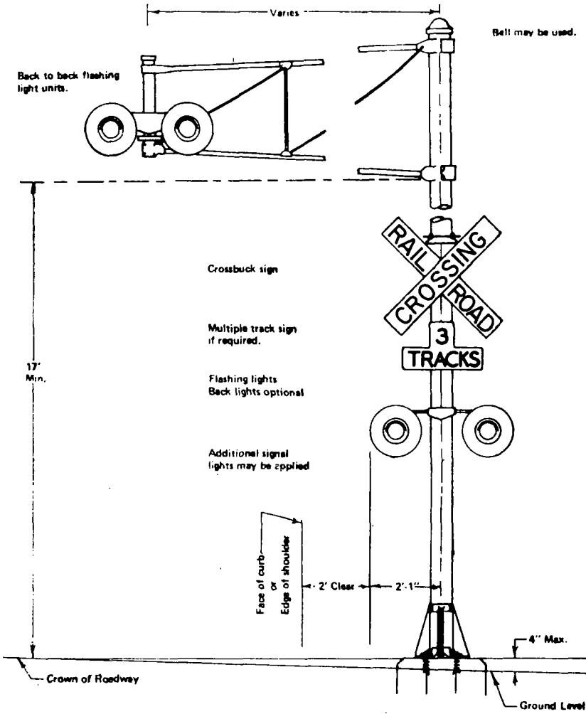
RAILROAD CROSSING SIGNAL CANTILEVER TYPE
