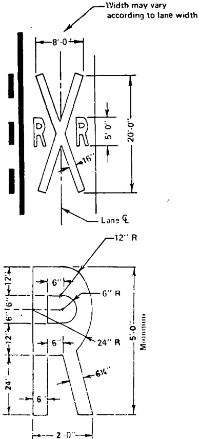
PAVEMENT MARKINGS MINNESOTA DEPARTMENT OF TRANSPORTATION
