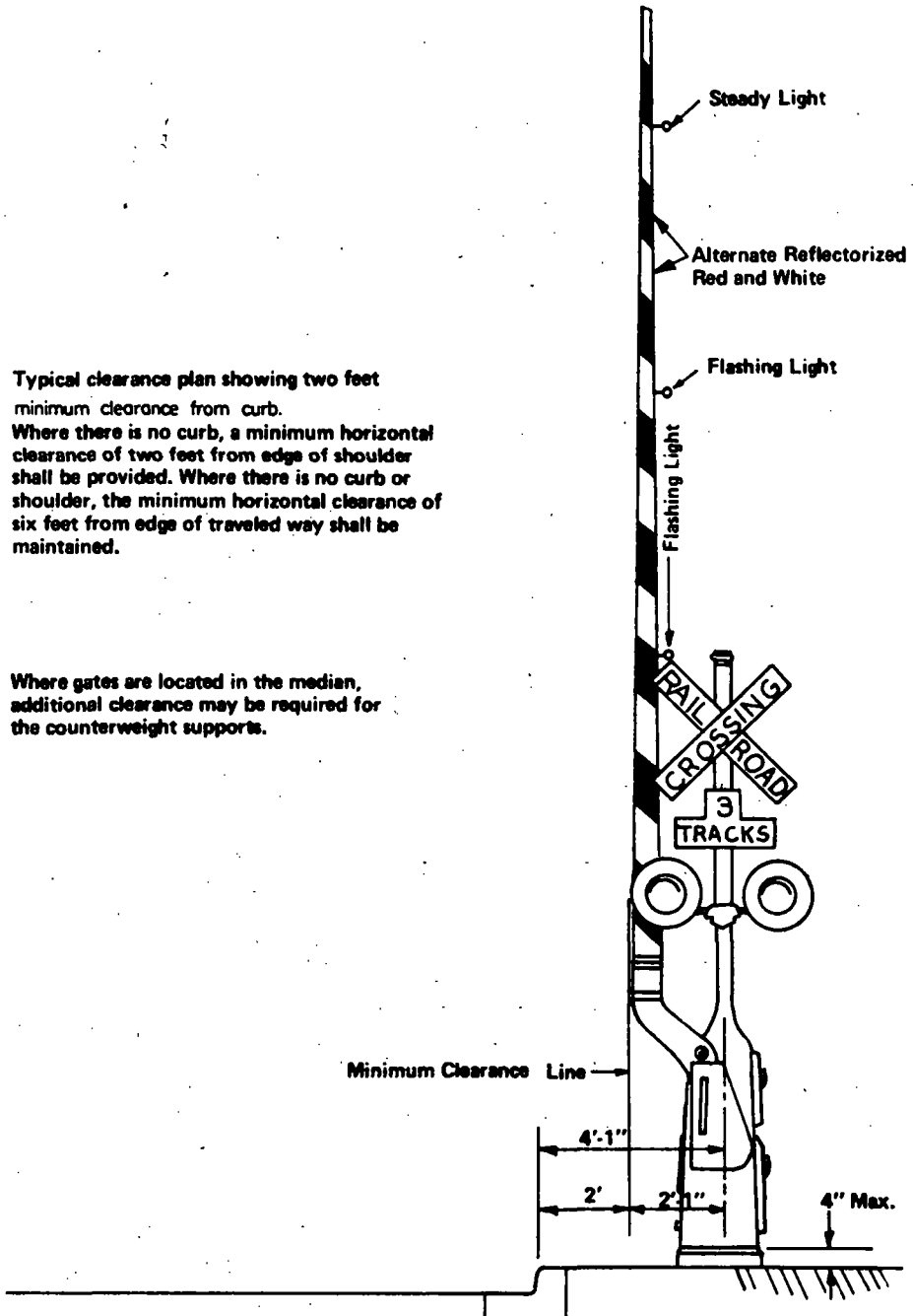
TYPICAL LOCATION PLAN FOR RAILROAD CROSSING SIGNALS WITH OR WITHOUT GATE
