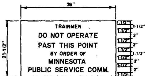
Type C-1
