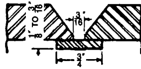
(a) BUTT JOINT WITH SPLIT BACKING RING
