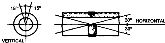
(Vertical Fixed Position-Horizontal Weld)
