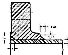
(b) FACE AND BACK WELD
