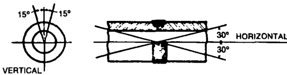
(Vertical Fixed Position-Horizontal Weld)
