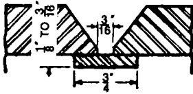
5230.1220 FIGURE 5: TYPICAL JOINTS WITH BACKING RING.
