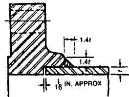
(c) SOCKET WELD FLANGE
