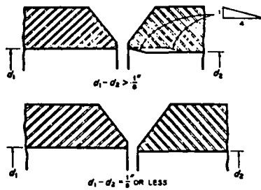
5230.1210 FIGURE 4: BUTT WELDING OF PIPES OR FITTINGS OF UNEQUAL WALL THICKNESSES.
