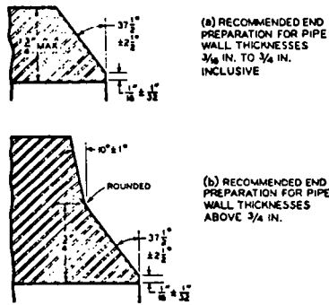
5230.1200 FIGURE 3: RECOMMENDED END PREPARATIONS.
