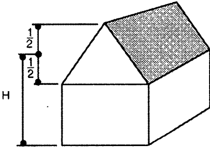
GABLE ROOF
