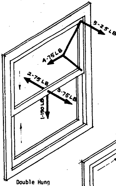
Double Hung
